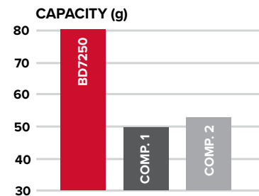
ISO 4548-12 Test: Flow Rate 28 gpm, ISO Medium Test Dust, Termination at 25 psid
