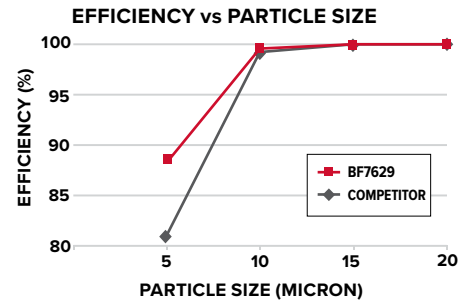
ISO 19438 Test: Flow Rate 3 gpm, ISO Medium Test Dust, 104°F, Termination at 5 psid
