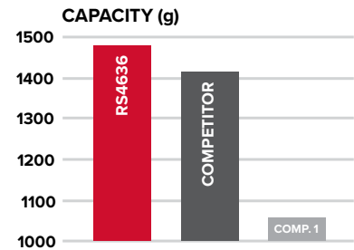
ISO 4548-12 Test: Flow Rate 28 gpm, ISO Medium Test Dust, Termination at 25 psid
